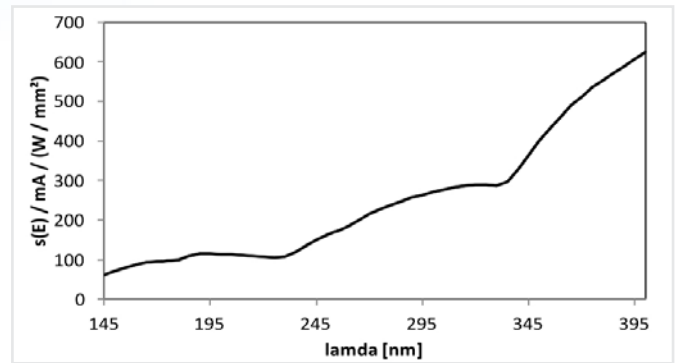
Typical, spectral sensitivy of the photo detector
